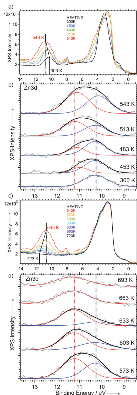
Figure 3. a, c) AP-XPS spectra (Zn 3d and Cu 3d regions) recorded at h\nu = 130 \text{ eV} in situ during MSR (0.12 mbar methanol + 0.24 mbar water) starting from CuZn \approx 10:1 . b, d) Corresponding Zn 3d peak deconvolution; red: BE \approx 11.2 \text{ eV} , Zn(ox); blue: BE \approx 10.25 \text{ eV} , bimetallic ZnCu. Details of Zn 3d binding energy and intensity trends are given in the Supporting Information, S2.
