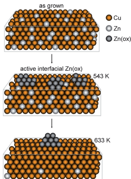
Scheme 1. Upper panel: pre-catalytic “as-grown” \text{CuZn} \approx 10:1 bimetallic state. Middle panel: superior “in situ” active surface state with maximum wetting of \text{Cu(Zn)}^0 by interfacial Zn(ox). Lower panel: High-temperature state after major Zn intensity loss by three-dimensional Zn(ox) clustering and/or bulk diffusion/desorption of \text{Zn}^0 .
